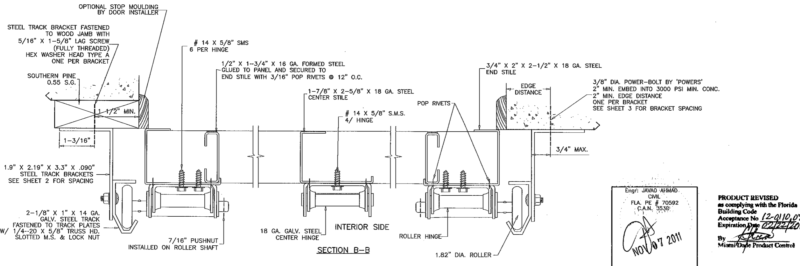
1ST SECTION (BOTTOM) REINFORCING
